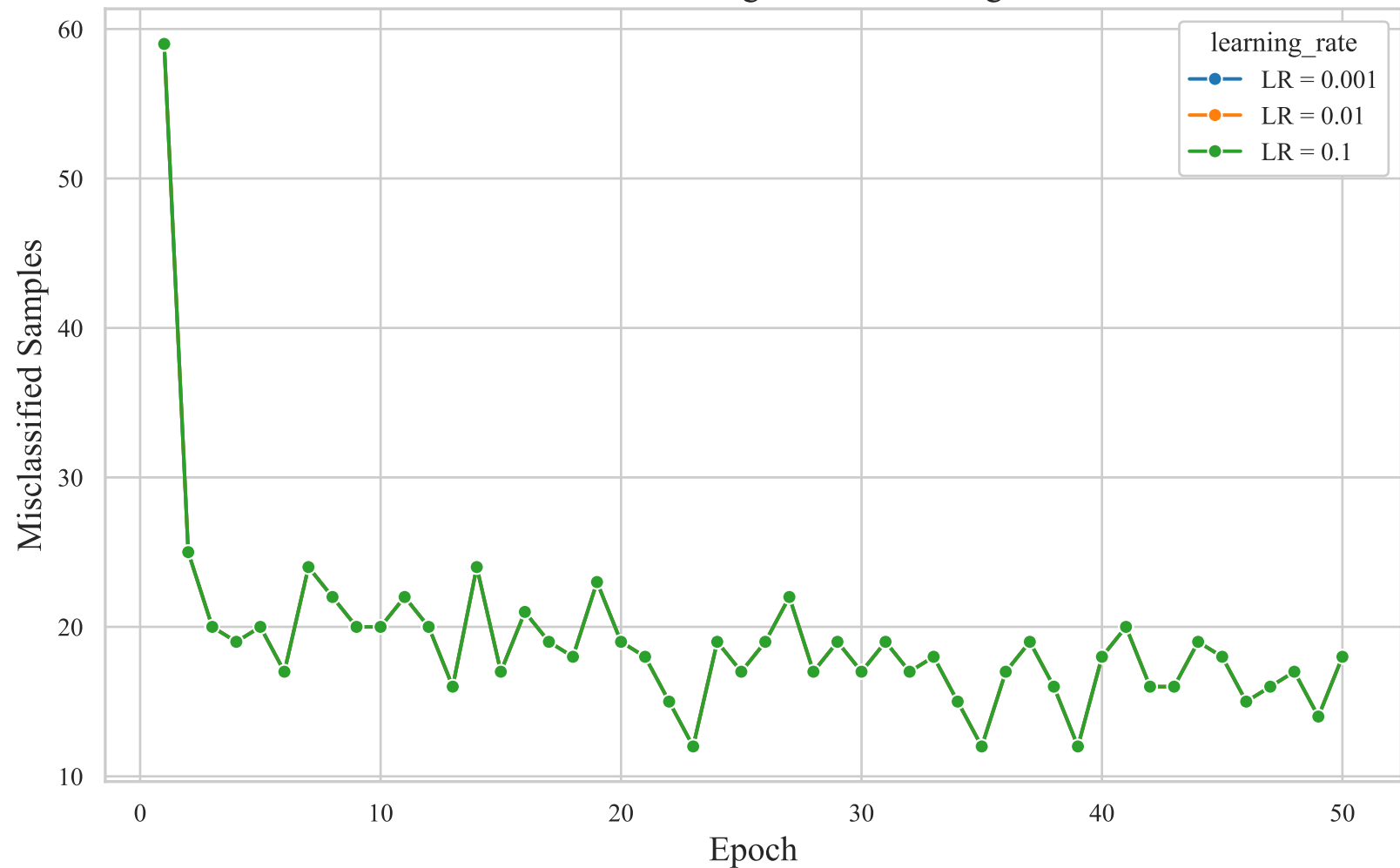
Effect of Learning Rate on Training
